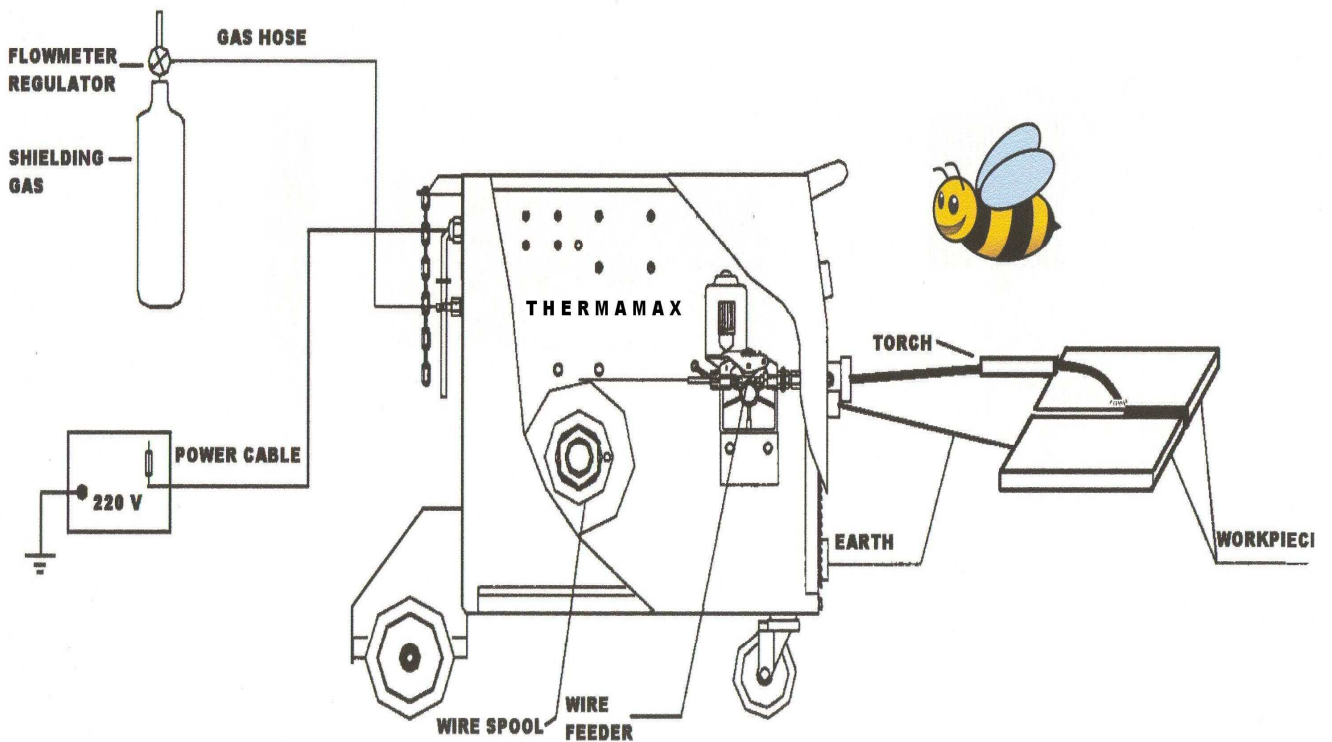
Connect Sketch (Compact Welder)
